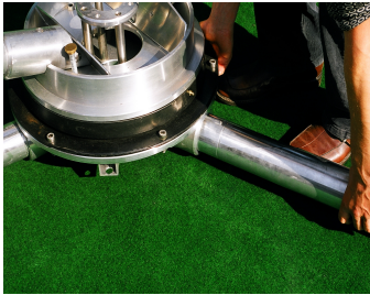
5. Introduce the legs until minimum check mark or further NO LESS!
