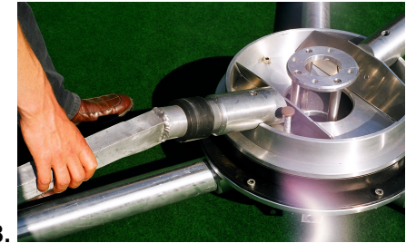
8. Introduce seat arm completely Close thread
